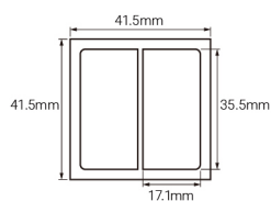
Duo color insert L35.5*W17.1mm
