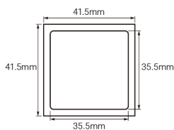
Single color insert L35.5*W35.5mm
